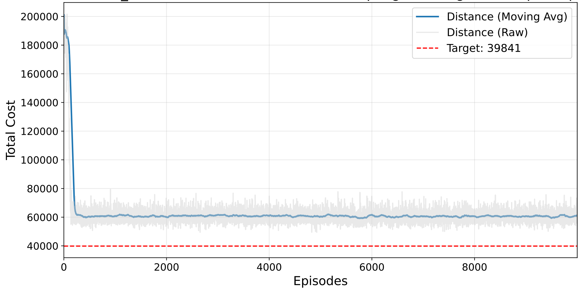
Final NO_MASK Masked AutoRL-SOP (Resampling) Training - kro124p.2.sop
